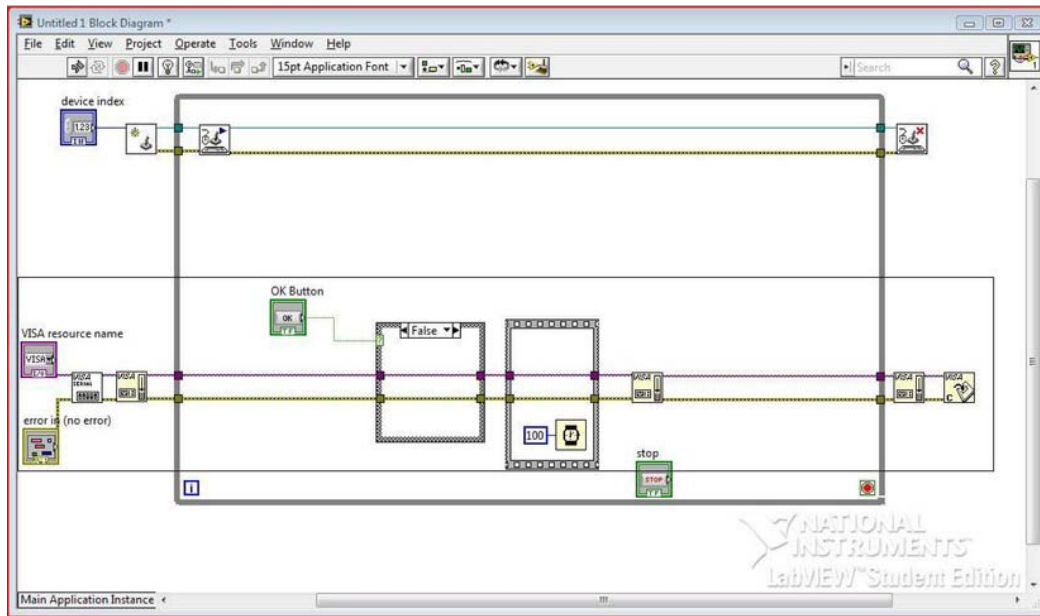
Figure 10-27. Make sure you wire the false condition of the Case Structure (part 2 of 2).
