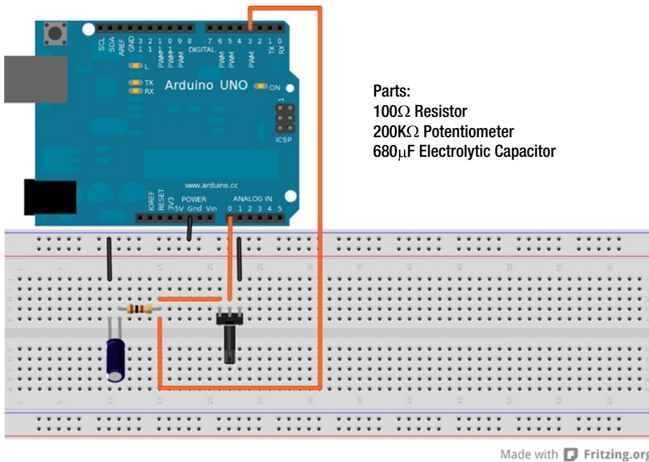
Figure 7-1. PID example circuit setup
