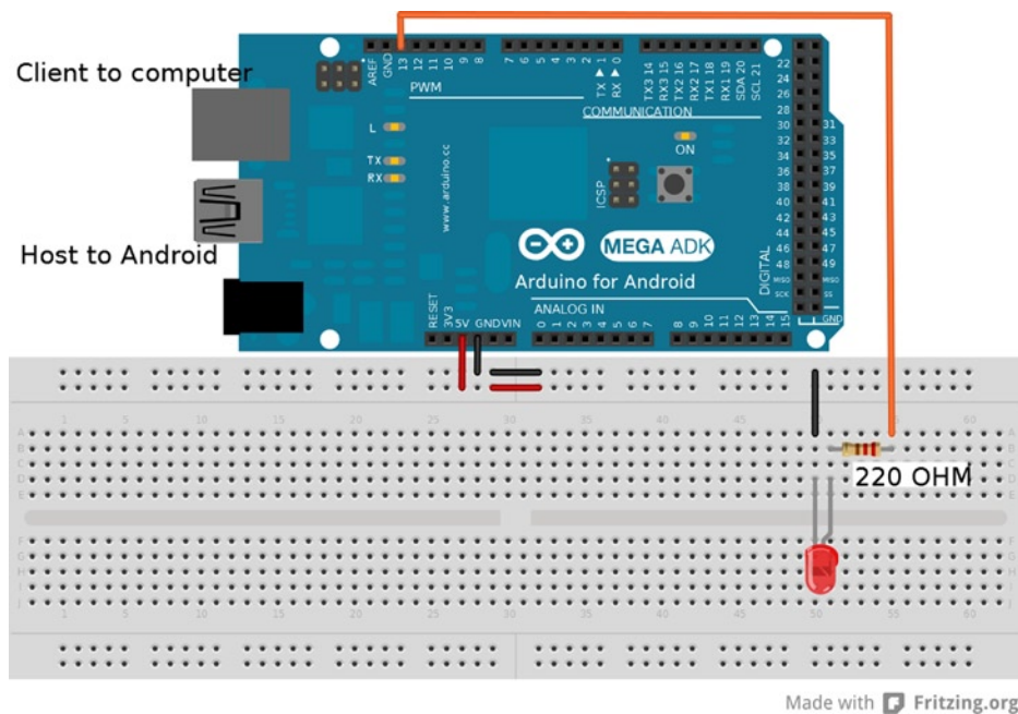
Figure 4-5. Arduino-to-Android configuration
