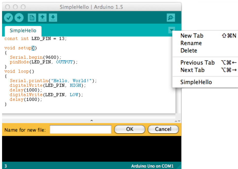
Figure 12-3. SimpleHello.ino sketch with “New Tab” option
