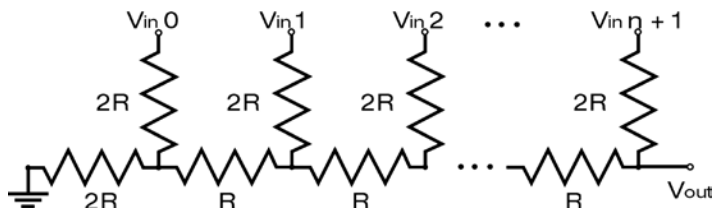
Figure 6-2. R-R2 ladder schematic
