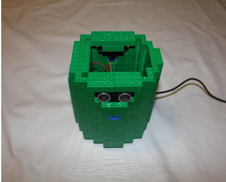
Figure 2-24. The layer above the ultrasonic sensors covers them
