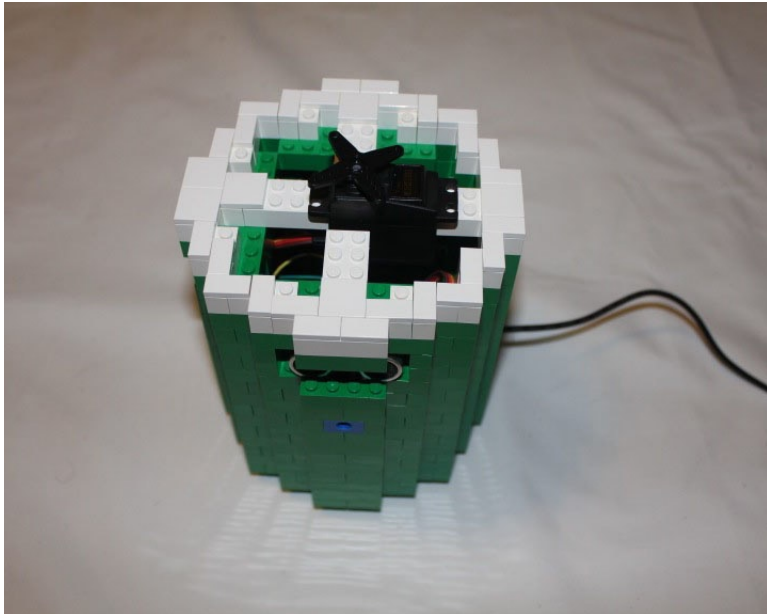
Figure 2-26. A layer of tiles is added to allow smooth movement of the head and to support the servo motor
