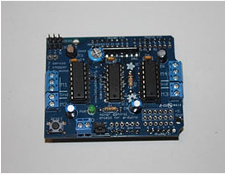
Figure 1-6. The assembled motor shield
