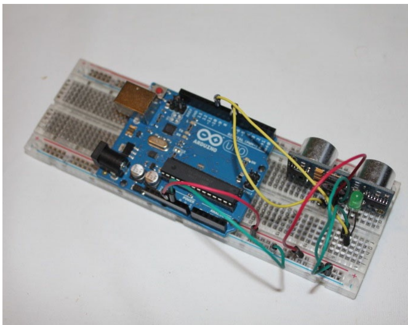
Figure 2-3. The Arduino, ultrasonic sensor, and green LED connected to the breadboard
